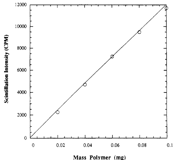
Figure 2. Mass coverage calibration for the tritium-labeled copolymer PVP-PS t52-63.
