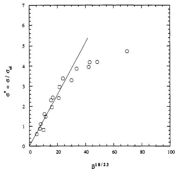
Figure 8. Normalized surface density \sigma^* versus \beta^{18/23} as measured by scintillation counting from tritium-labeled adsorbed layers (squares) and XPS (circles). The solid line represents a least-squares fit to the linear portion of the data (excluding five data points at highest \beta values) as predicted from eq 13.
